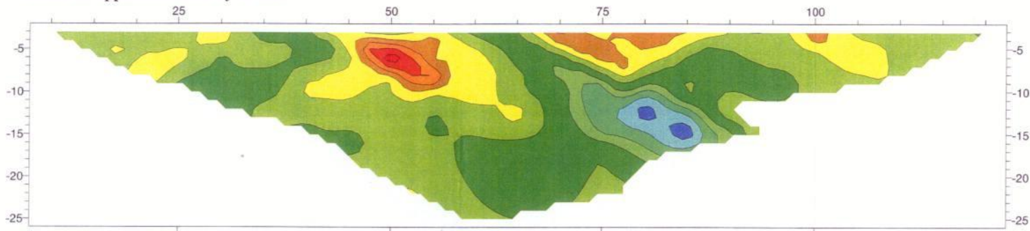
Measured apparent resistivity section
