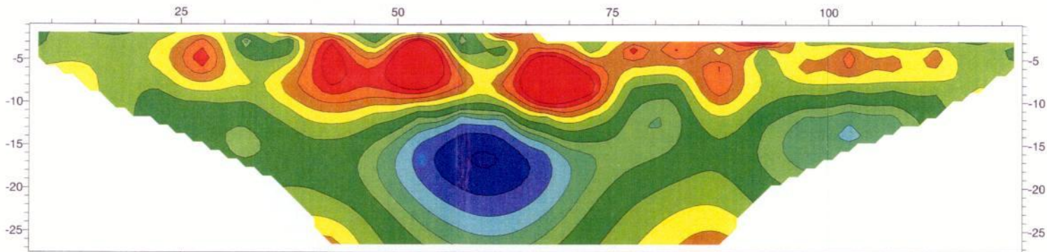
Model resistivity section - 6.3% Inversion RMS error
