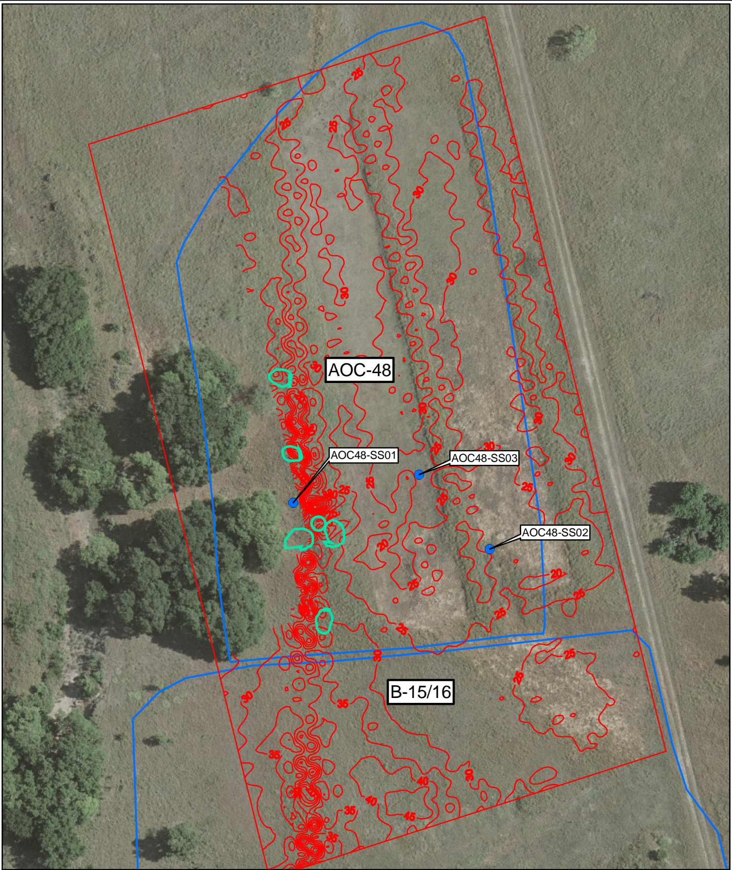
Figure AOC48-11 SWMU AOC-48 Sample Locations and Test Pit Map PARSONS
