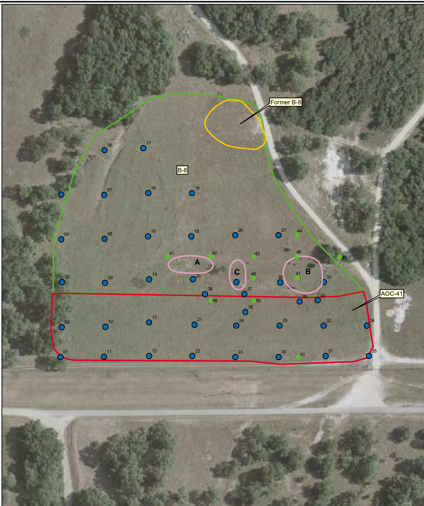
Figure AOC41-7 Soil Gas and Geophysical Anomaly Map Camp Stanley Storage Activity PARSONS
