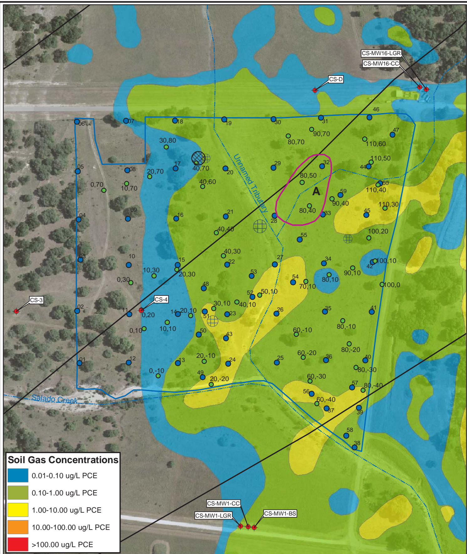
Figure AOC38-8 SWMU AOC-38 Soil Sample and Geophysical Anomaly Location Map, with PCE Soil Gas Contours PARSONS
